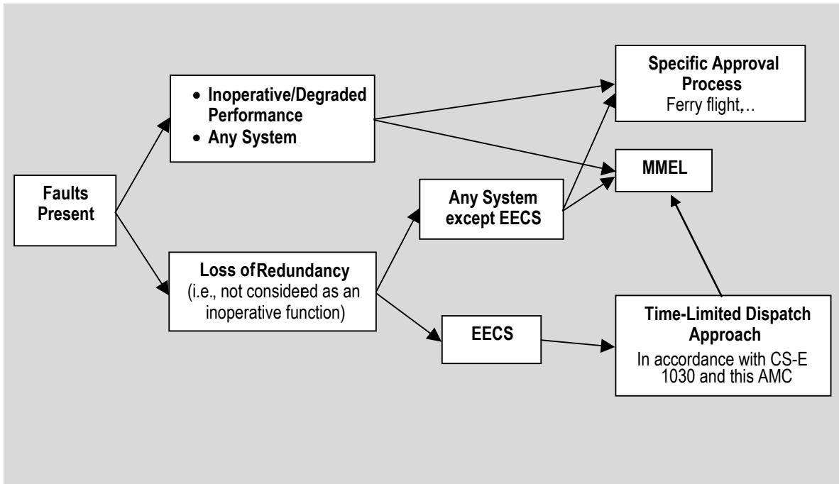
Figure 2: Different possible ways of managing Dispatch with Engine Faults
