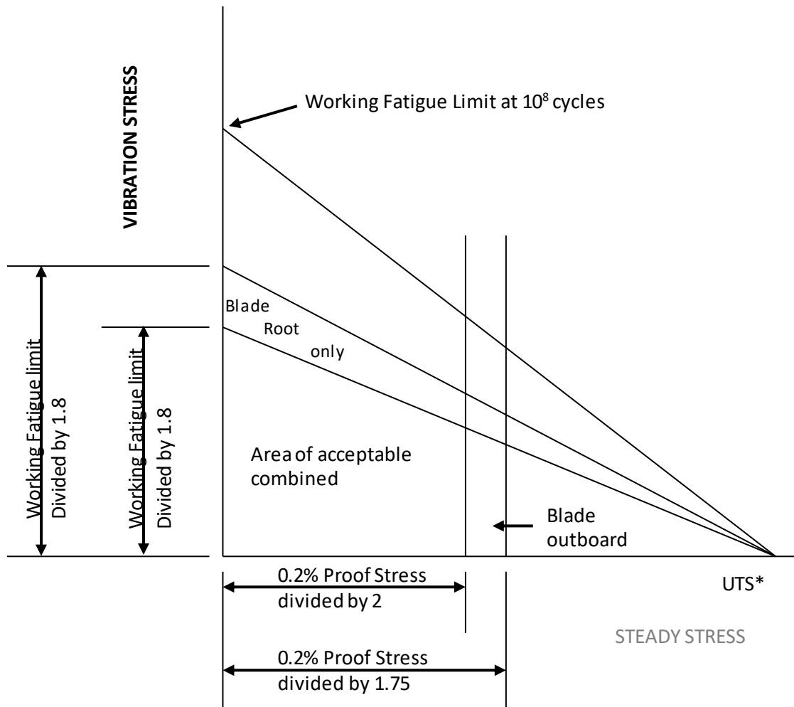
FIGURE 1 ACCEPTABLE STRESS LEVELS FOR CONVENTIONAL PROPELLERS WITH SOLID ALUMINIUM ALLOY BLADES
