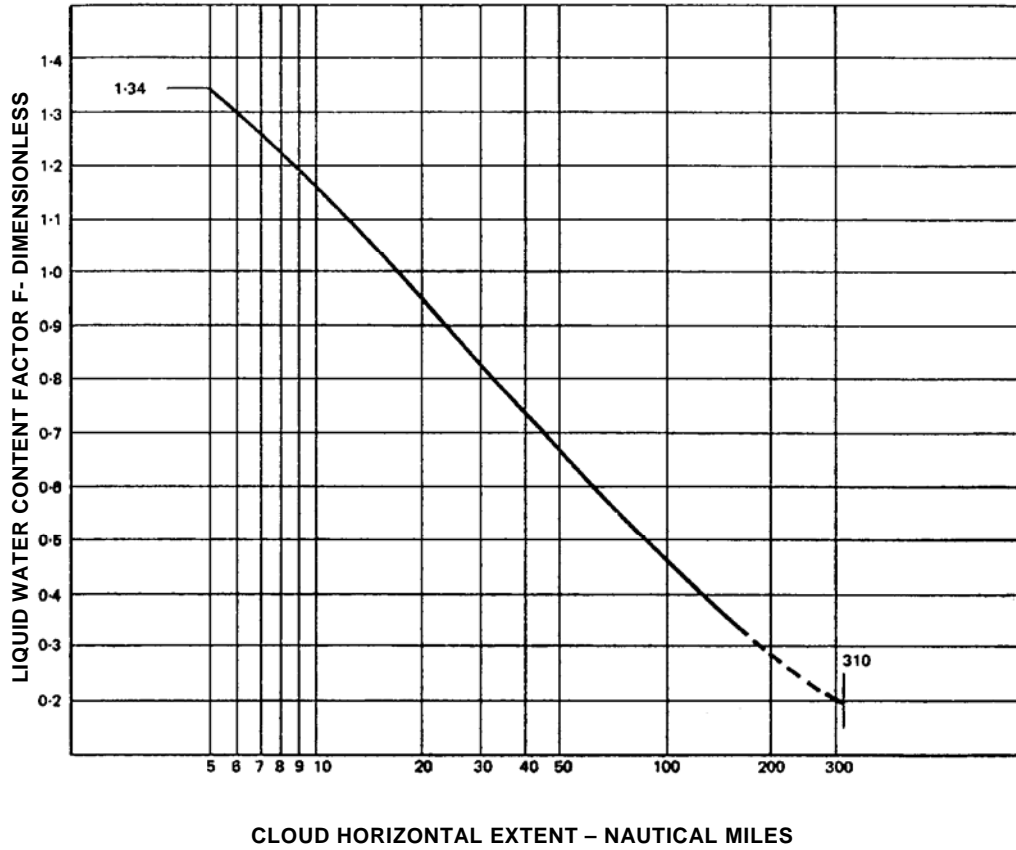
CONTINUOUS MAXIMUM (STRATIFORM CLOUDS) ATMOSPHERIC ICING CONDITIONS LIQUID WATER CONTENT FACTOR VS CLOUD HORIZONTAL DISTANCE Figure 4
