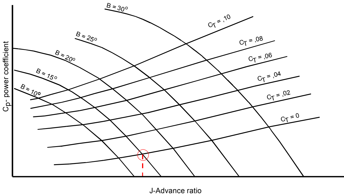
Figure 17-2 PROPELLER COEFFICIENTS
