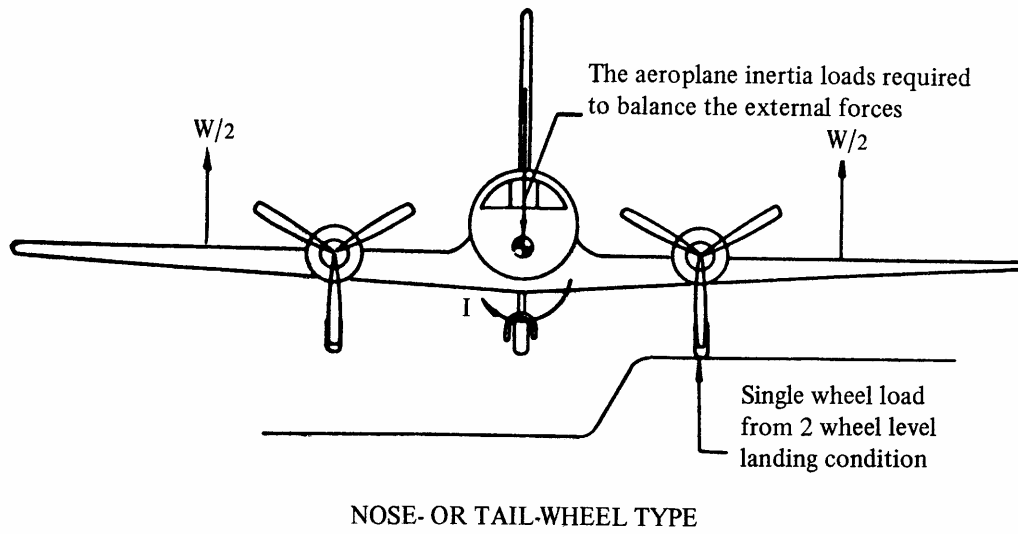
FIGURE 4 ONE-WHEEL LANDING
