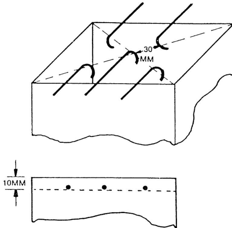
FIGURE 5. THERMOCOUPLE POSITION
