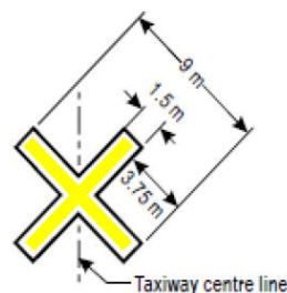
Illustration b) Closed taxiway marking
