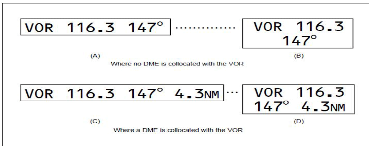
Figure N-7. VOR aerodrome check-point sign
