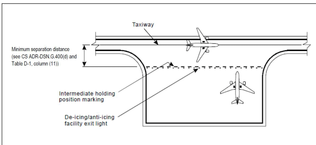
Figure M-11. Example of remote de-icing/anti-icing facility
