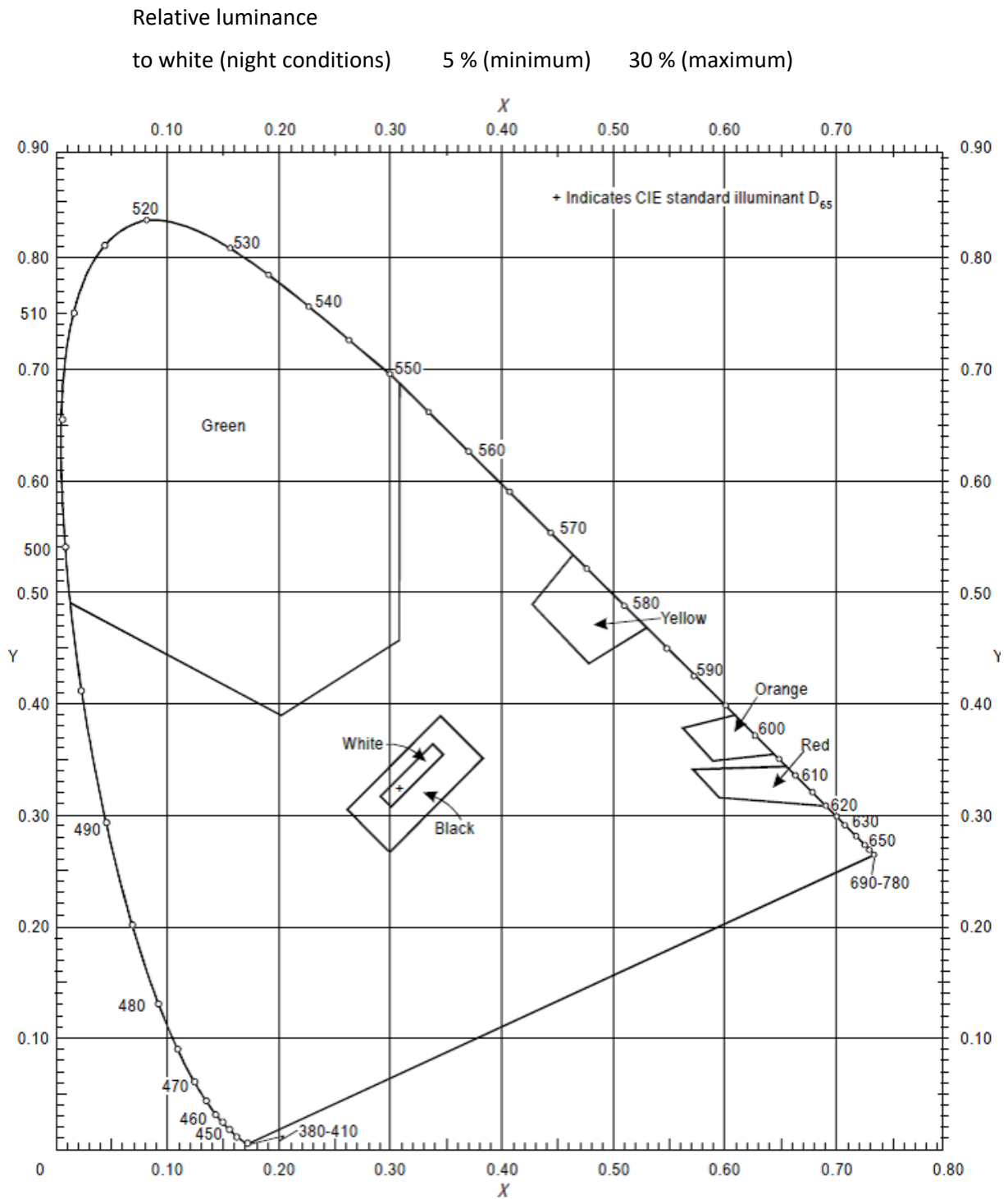
Figure U-2. Ordinary colours for markings and externally illuminated signs and panels
