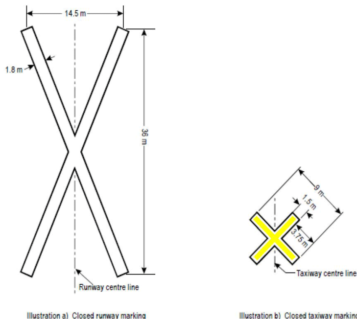
Figure R-1. Runway and taxiway closed markings
