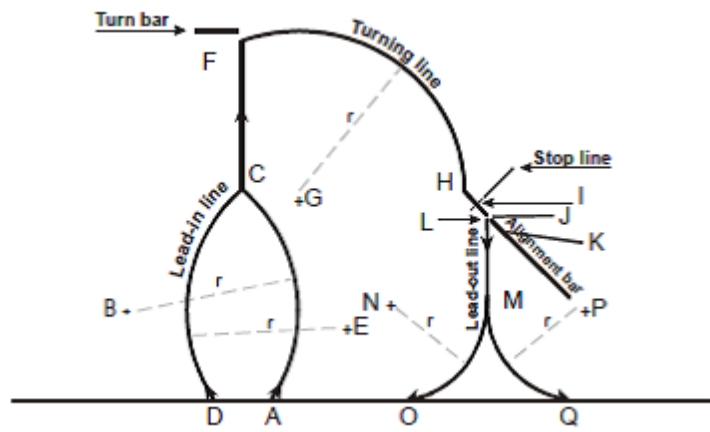
Figure 12 - Turning lines
