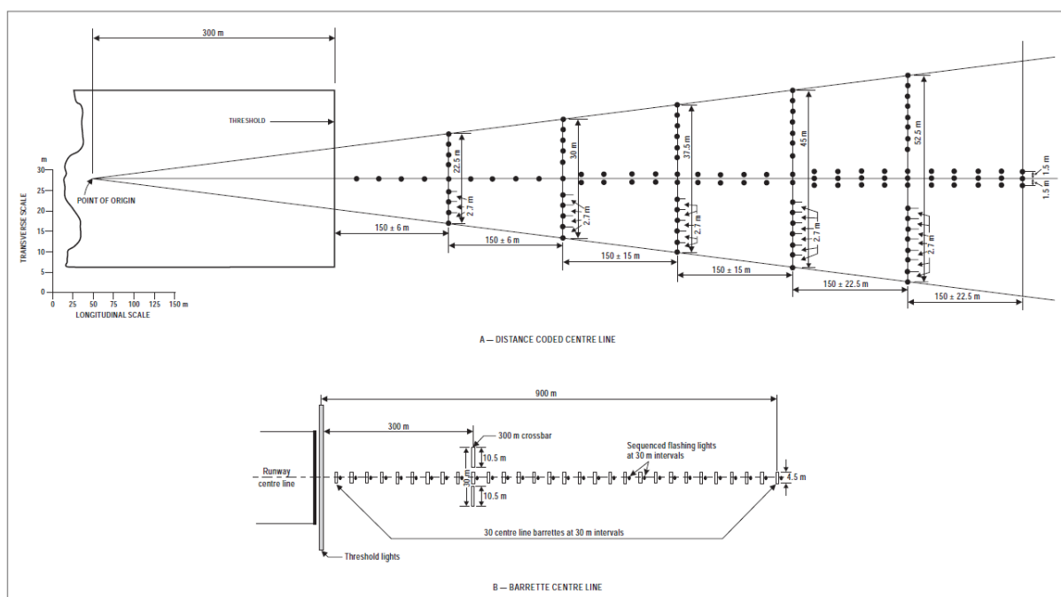
Figure M-2. Precision approach Category I lighting systems
