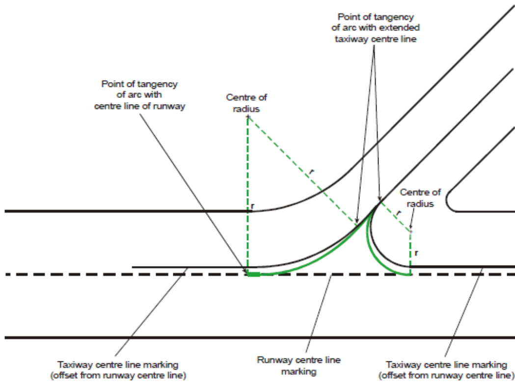
Figure 5 - Runway and taxiway intersections to be surveyed
