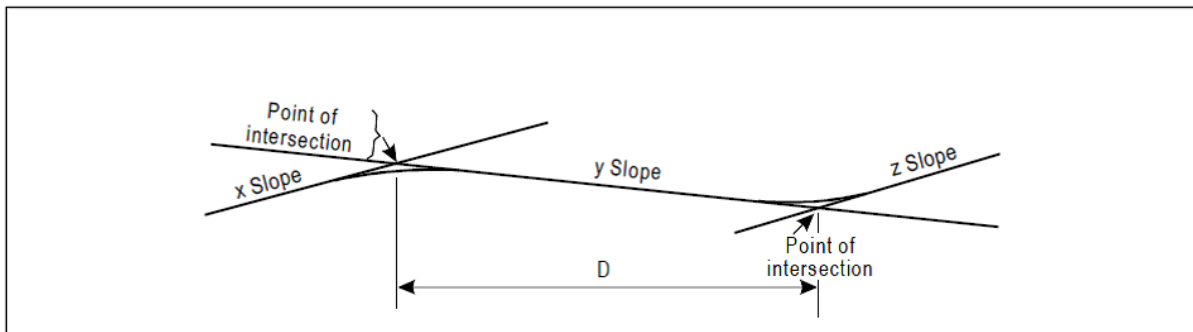
Figure GM-B-2. Profile on centre line of runway
