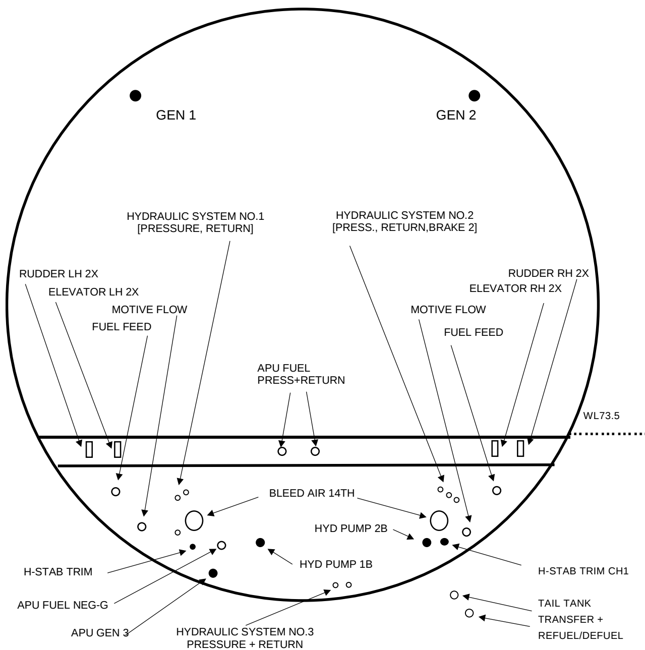
TYPICAL LAYOUT OF SYSTEMS IN ROTOR PLANE
