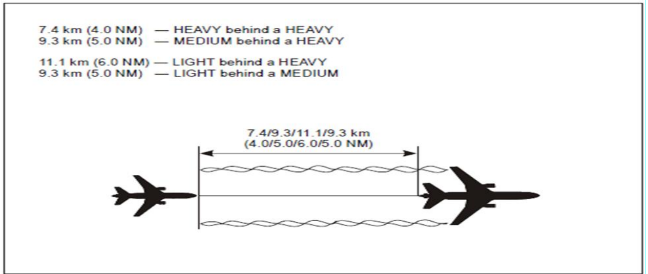
Figure 48: Operating directly behind
