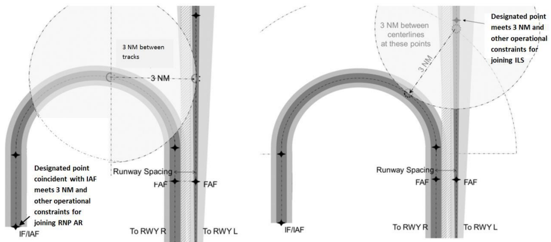
Figure 59: Established on RNP AR APCH concept
