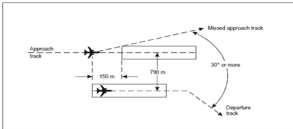
Figure 58: Segregated parallel operations where runways are staggered
