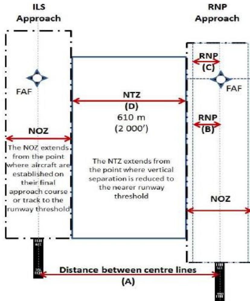
Figure 51: Distance between centre lines, NTZ and NOZ
