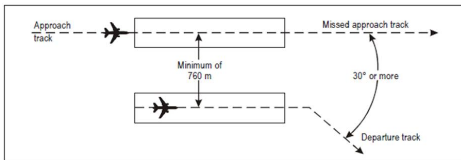
Figure 56: Segregated parallel operations
