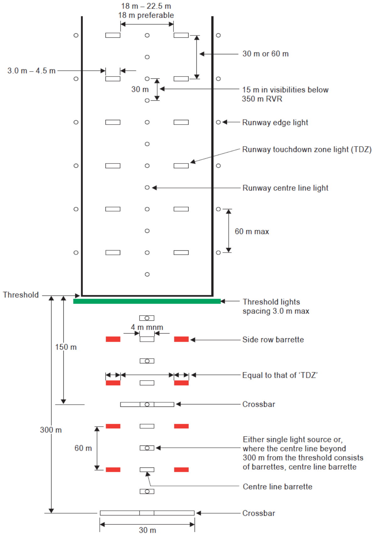
Figure M-3B. Inner 300 m approach and runway lighting for precision approach runways,
