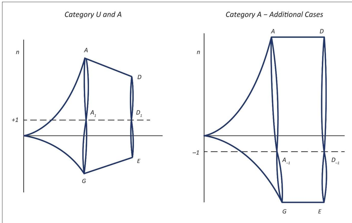
Figure 3 PITCHING MANOEUVRES
