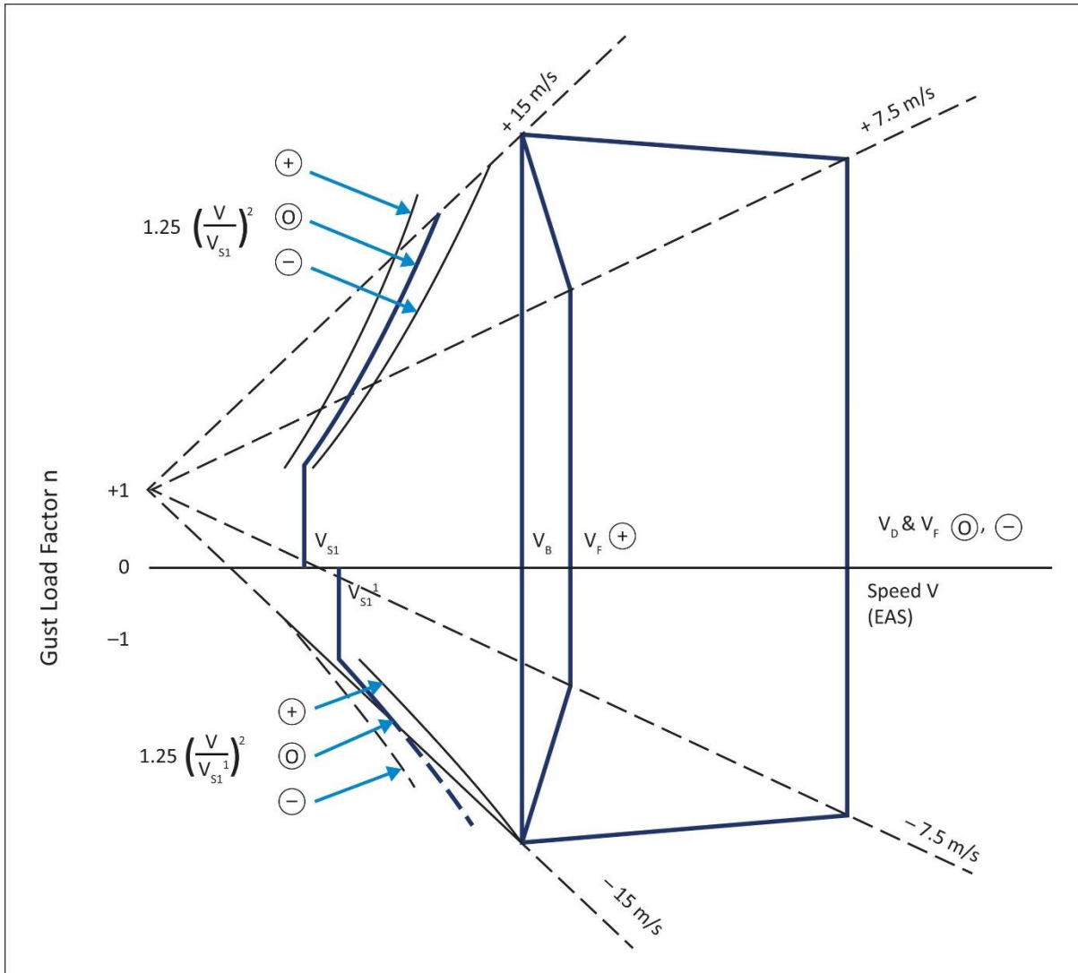
Figure 2 GUST ENVELOPE
