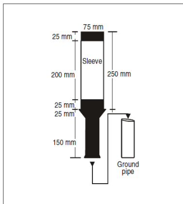
Figure GM-P-1. Taxiway edge marker
