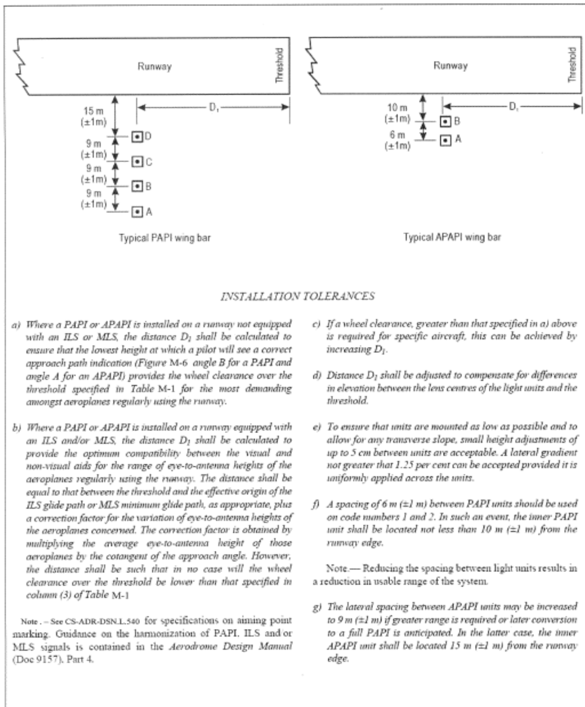
Figure M-4. Siting of PAPI and APAPI
