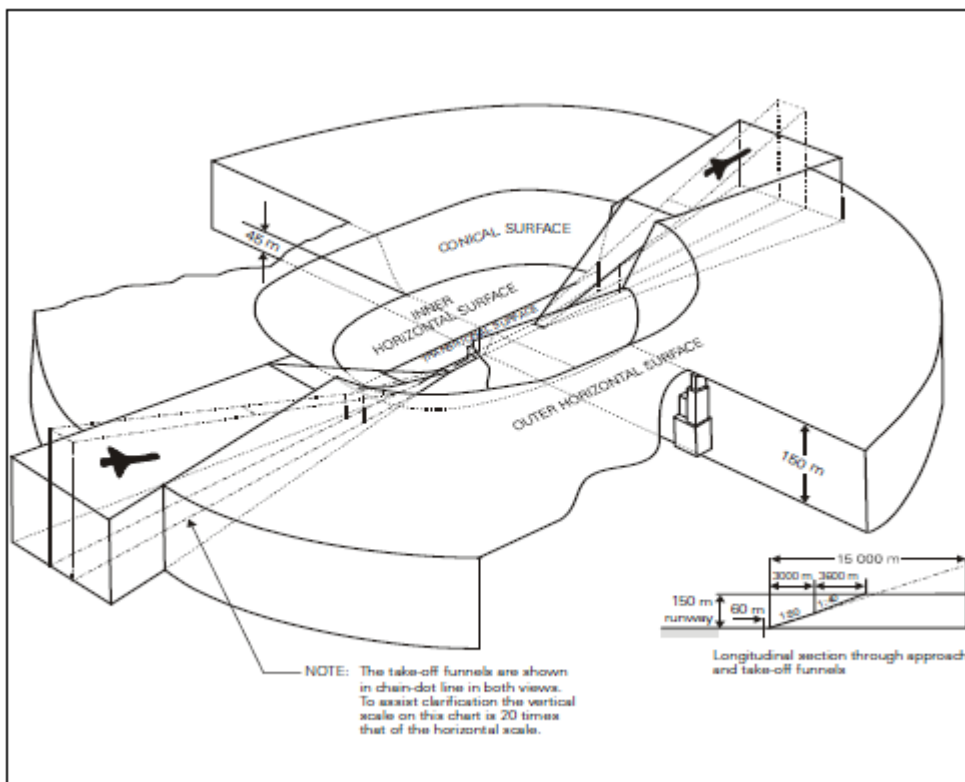
Figure GM-H-1 Disposition of Outer Horizontal Surface
