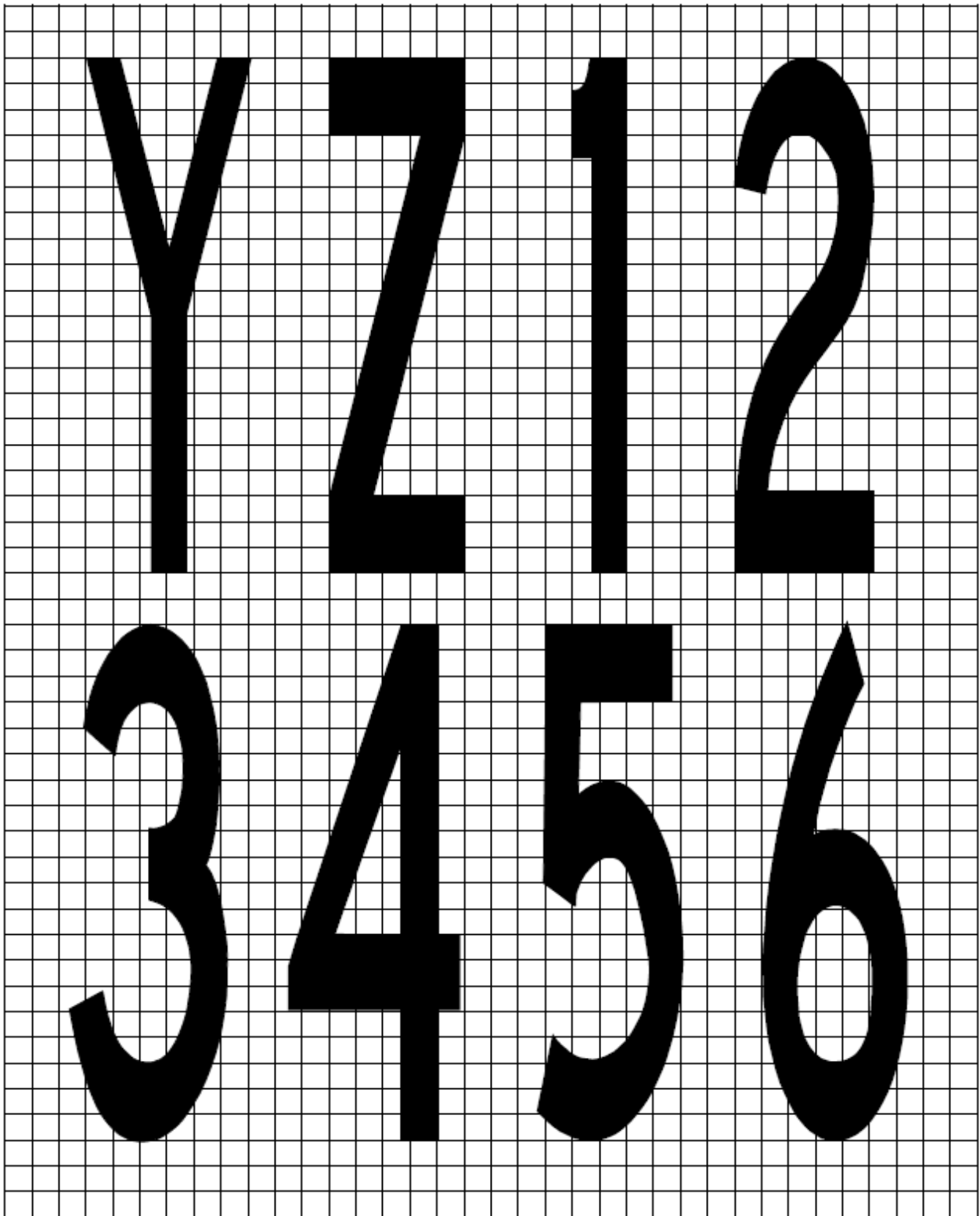
Figure L-10D. Mandatory instruction marking inscription form and proportions
