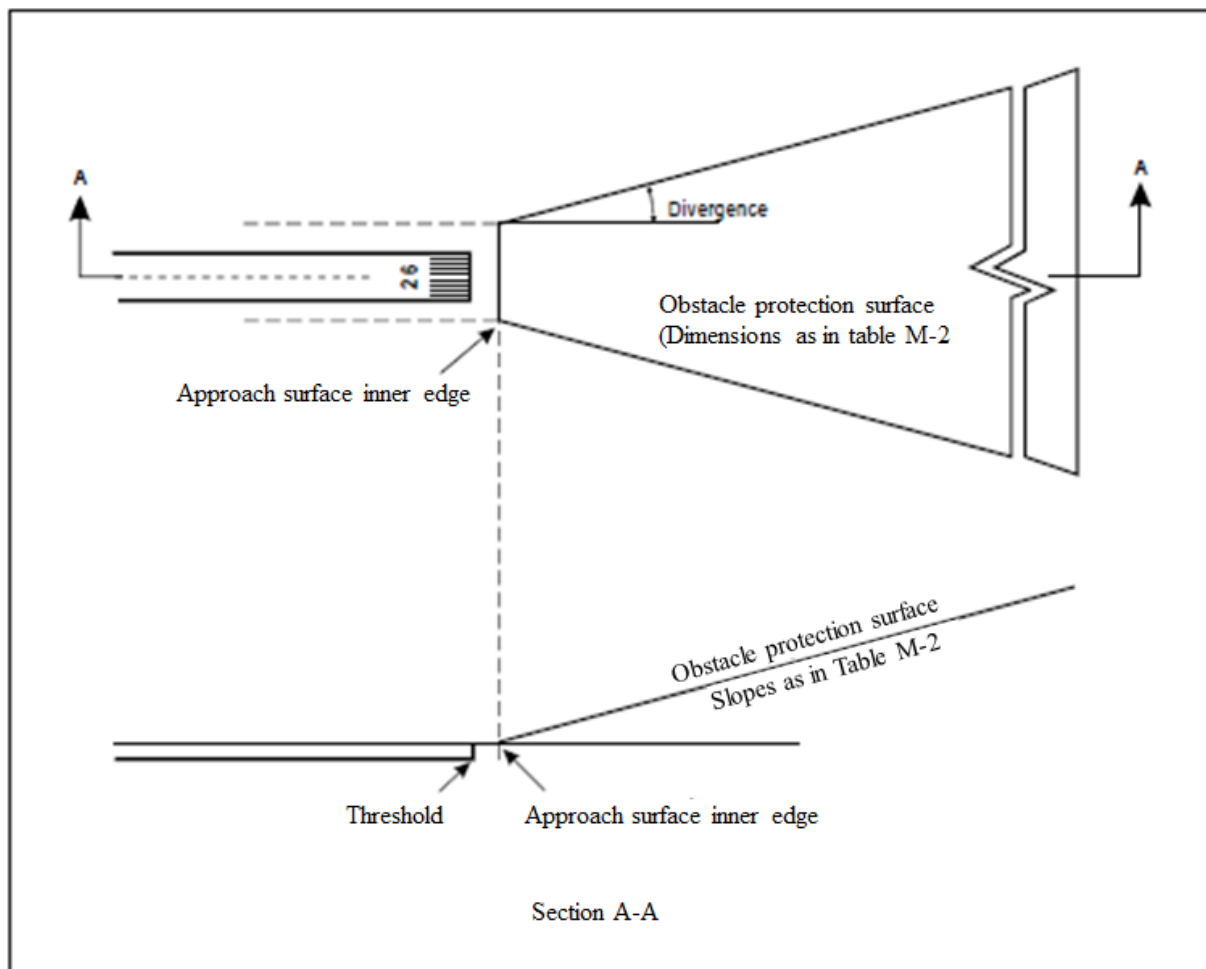
Figure M-6. Obstacle protection surface for visual approach slope indicator systems
