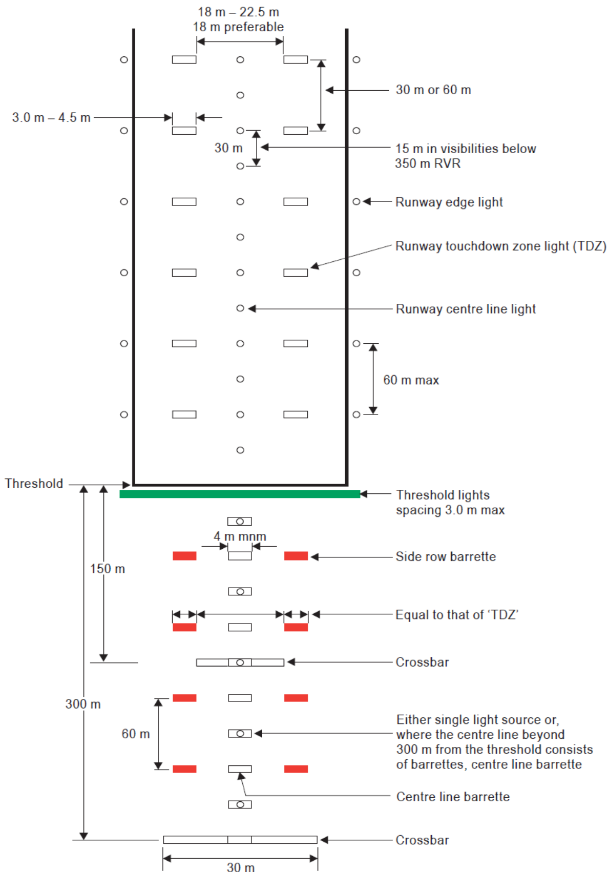
Figure M-3B. Inner 300 m approach and runway lighting for precision approach runways, categories II and III
