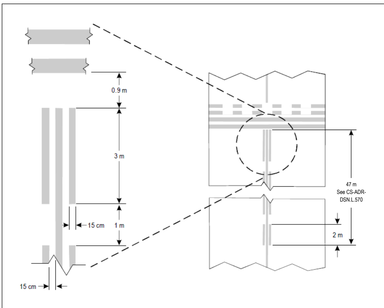
Figure L-6. Enhanced taxiway centre line marking
