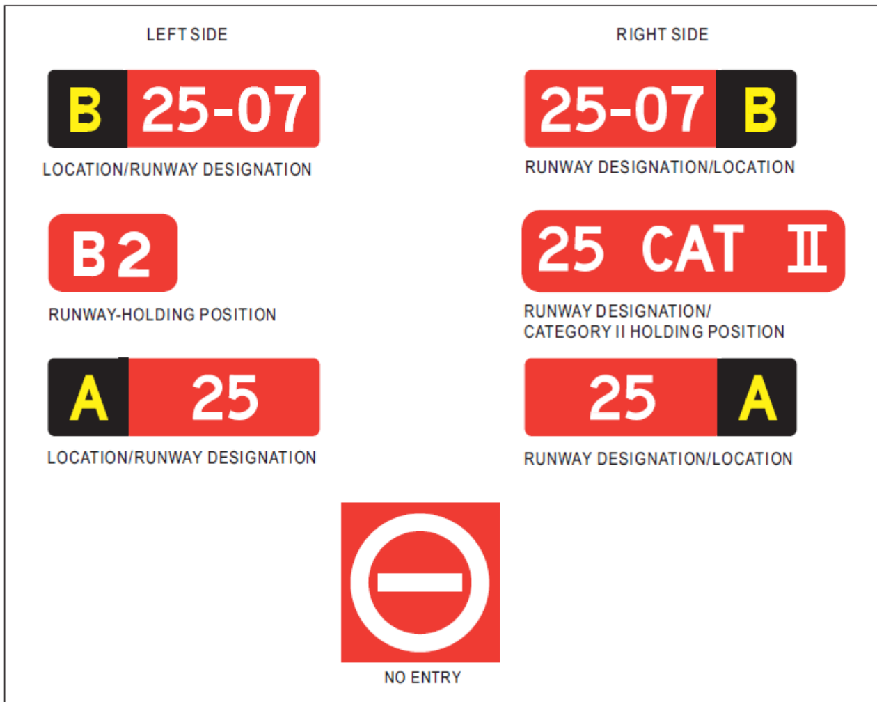
Figure N-4. Mandatory instruction signs
