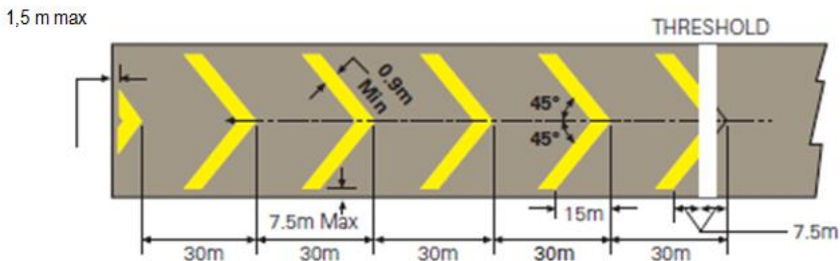
Figure R-2. Pre-threshold area marking
