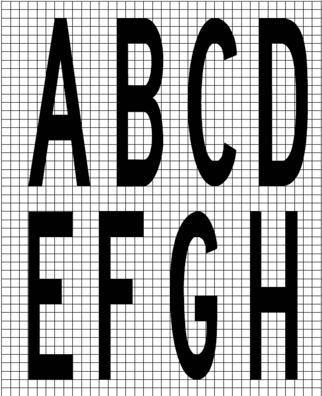
Figure L-10A. Mandatory instruction marking inscription form and proportions
