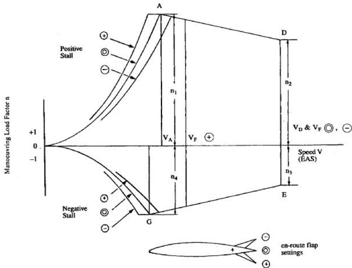
FIGURE 1 MANOEUVRING ENVELOPE
