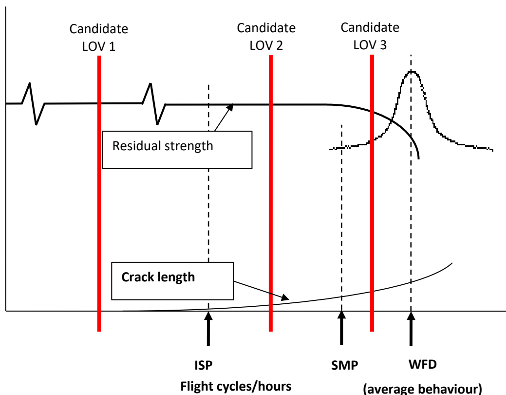
Figure 2-1: Comparison of WFD-susceptible structure to aircraft LOV
