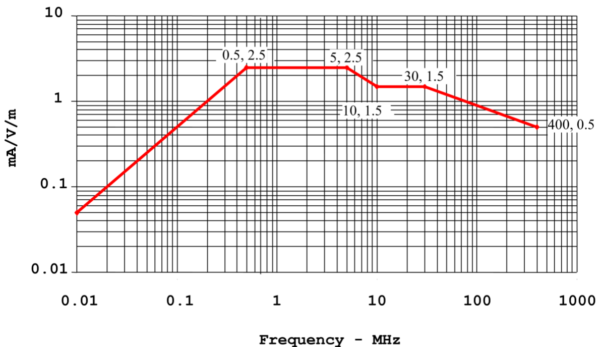
Figure A1-5: Generic transfer function — All aircraft
