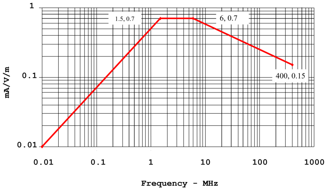
Figure A1-2: Generic transfer function — Aeroplanes
