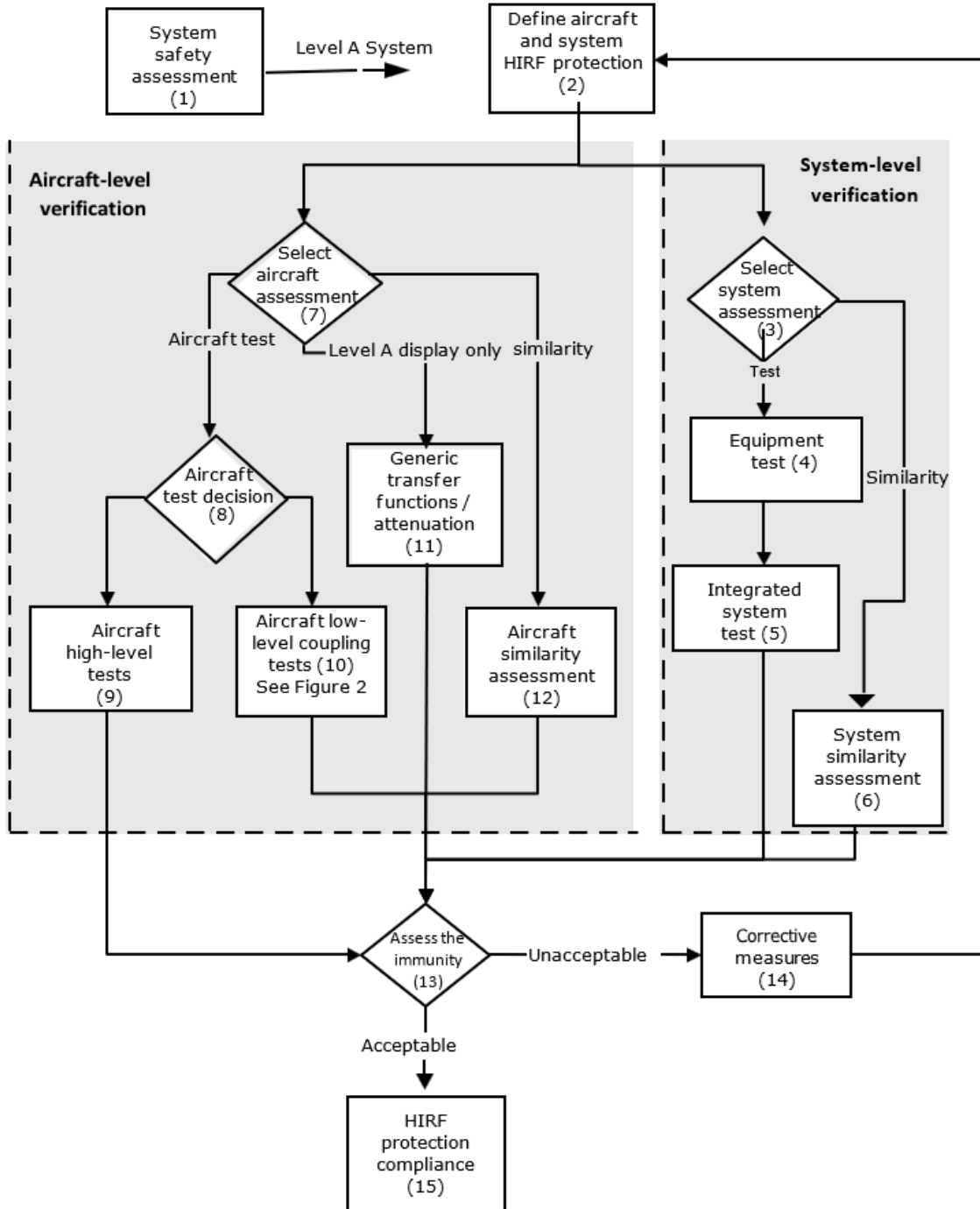
Figure 1: Routes to HIRF compliance — Level A systems
