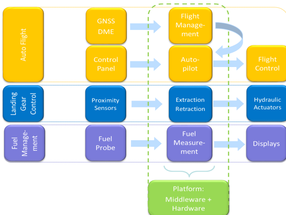
Figure 3 — Illustration of an IMA architecture
