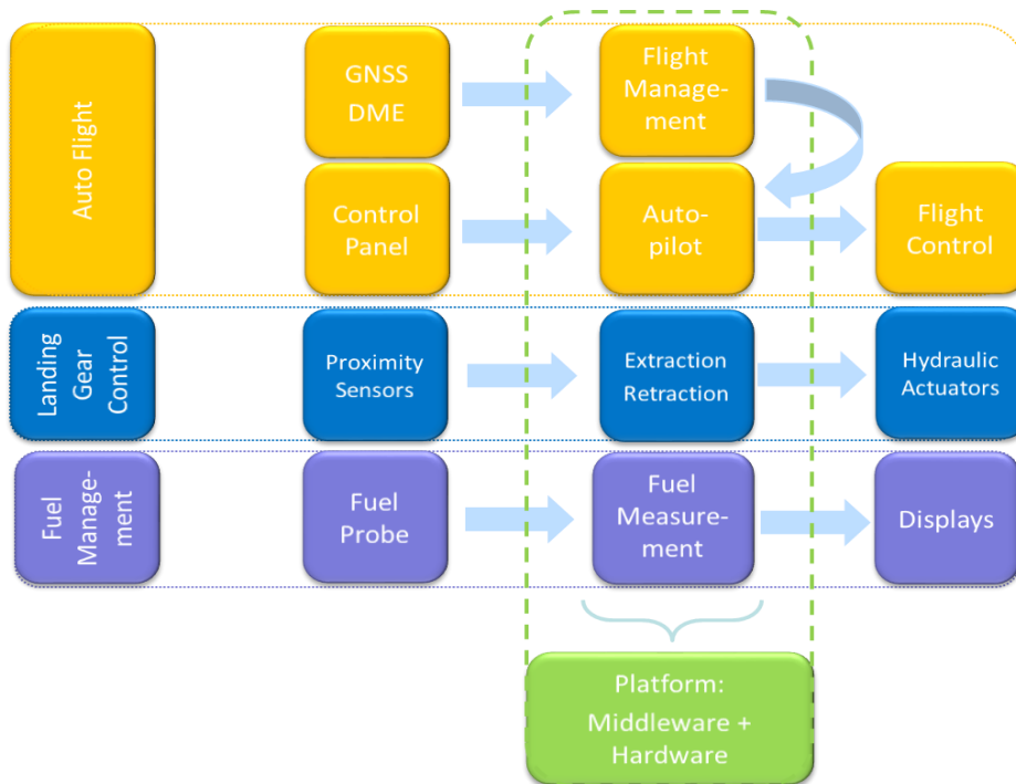
Figure 3 — Illustration of an IMA architecture
