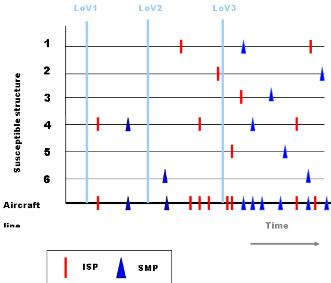
Figure 2-2: Aeroplane maintenance actions [Amdt 20/20] [Amdt 20/22]
