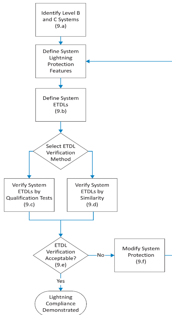
Figure 3 — Typical compliance process for Level B and C systems
