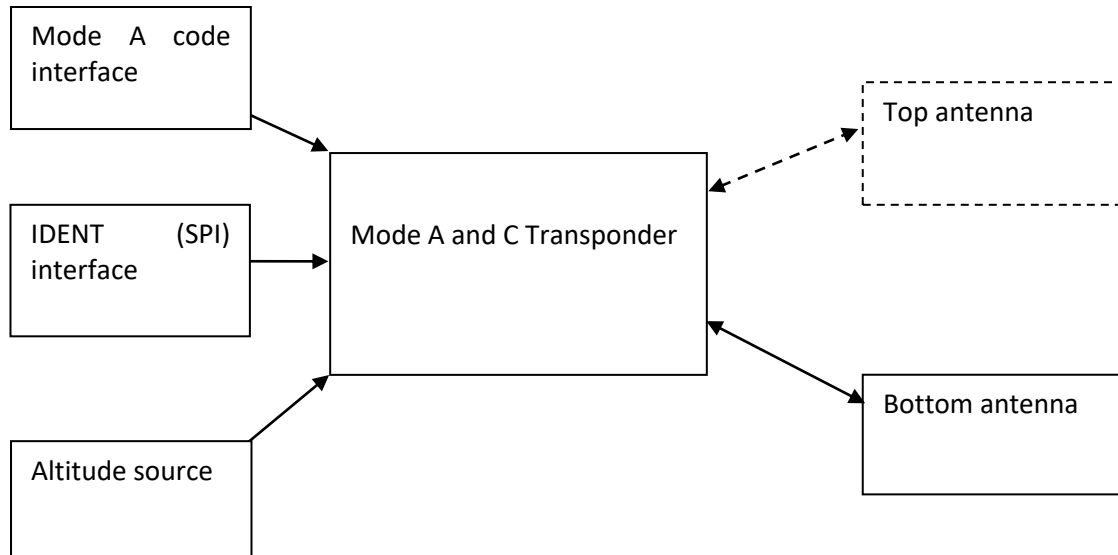
Figure 2: Mode A/C transponder interfaces
