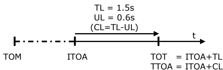
Figure 1: Latency Parameters
