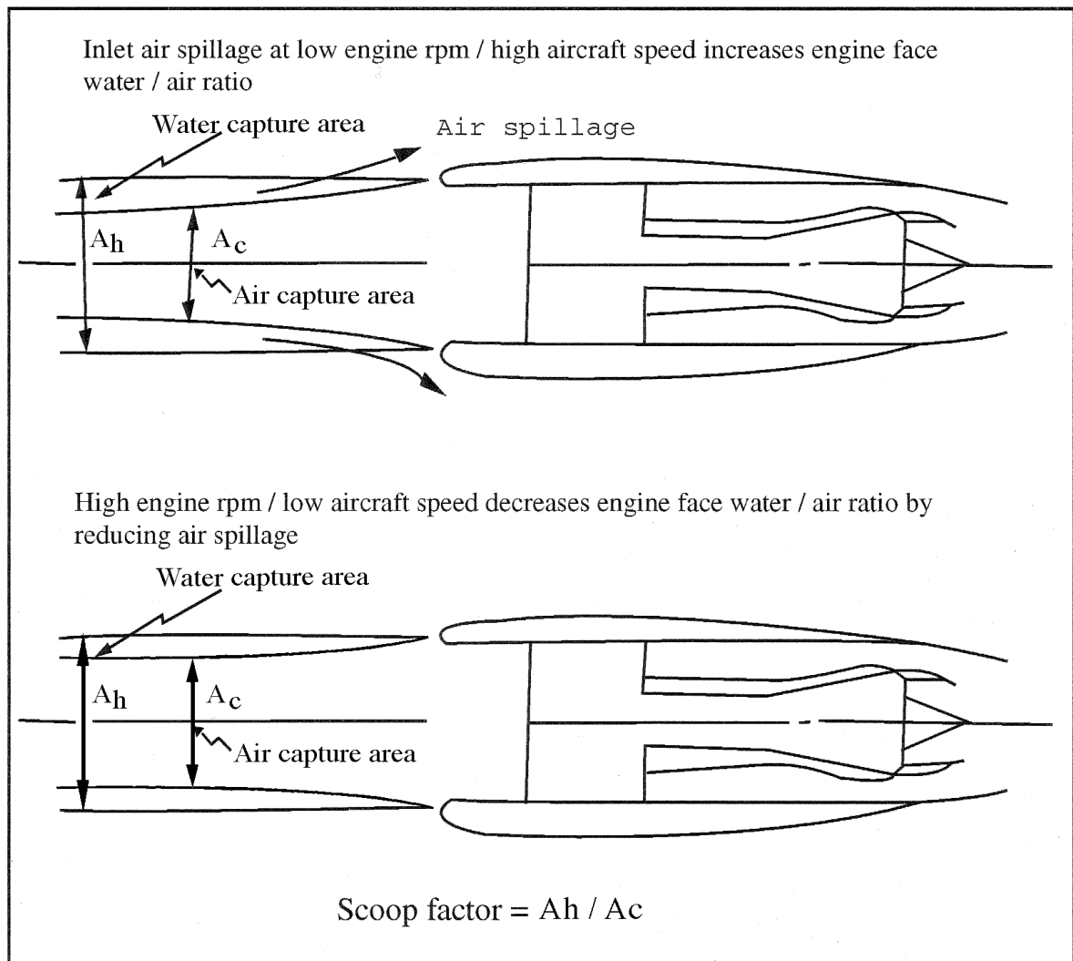
Figure 1 Scoop Factor
