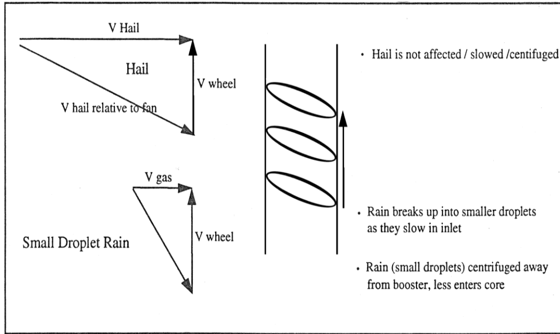
Figure 2 Velocity Vector Diagram
