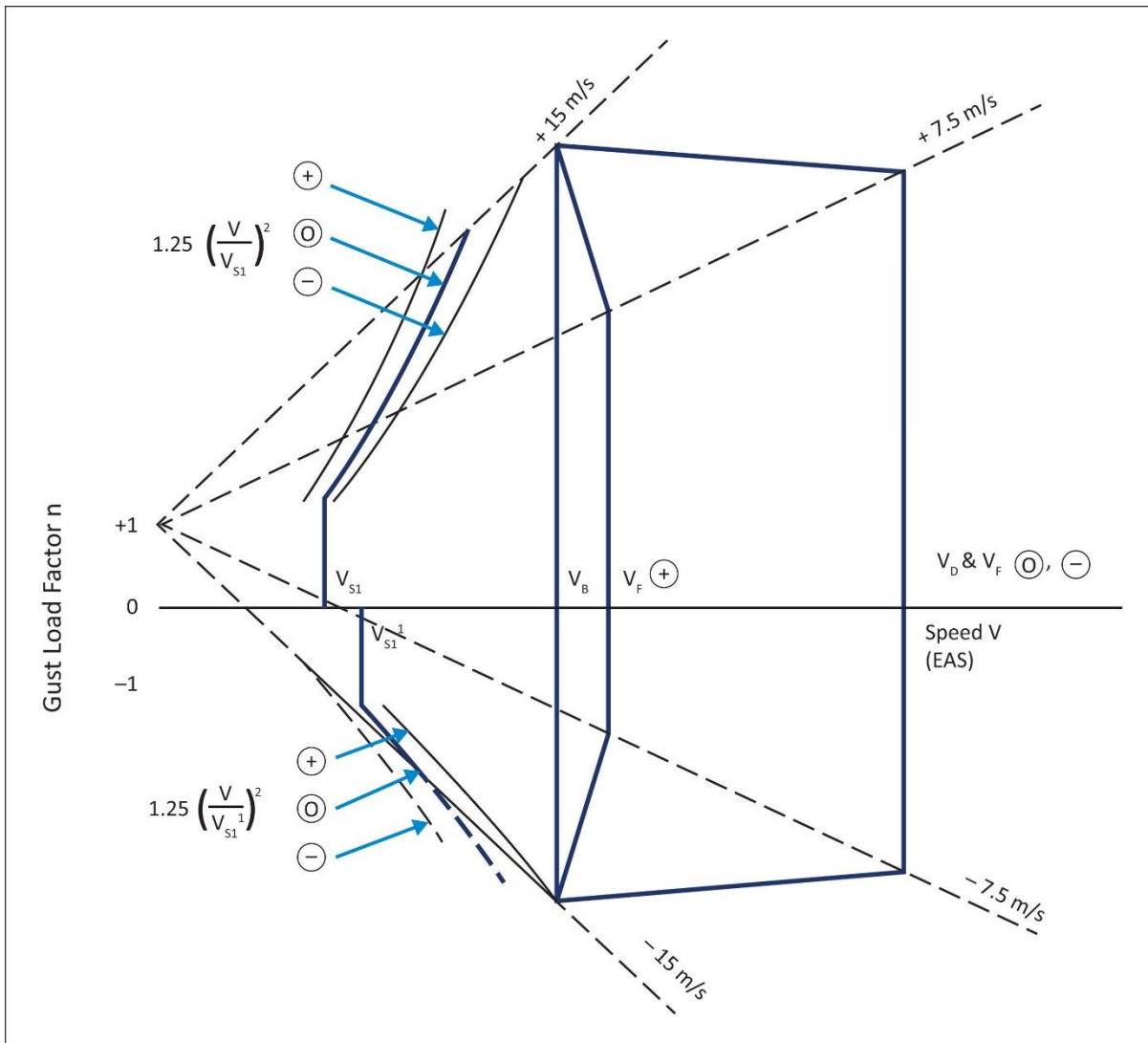
Figure 2 GUST ENVELOPE
