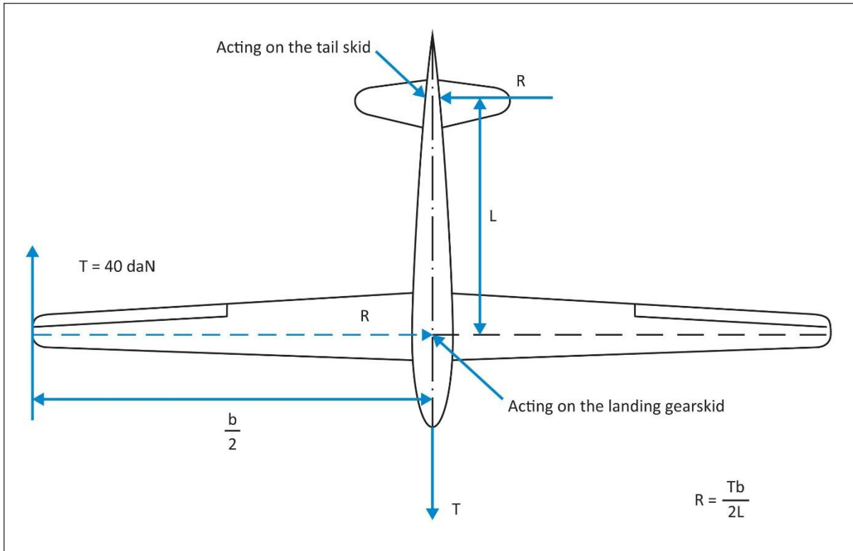
Figure 4 WING-TIP LANDING
