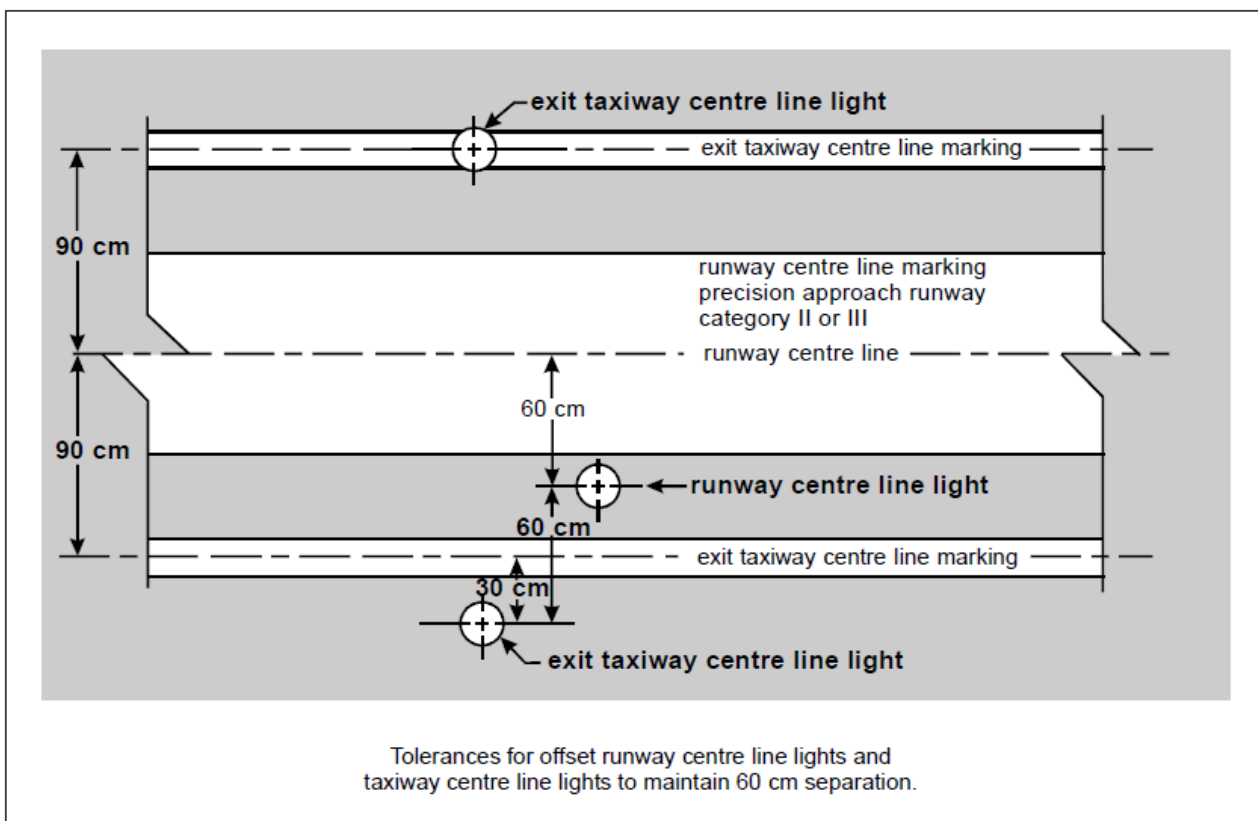
Figure M-10. Offset runway and taxiway centre line lights
