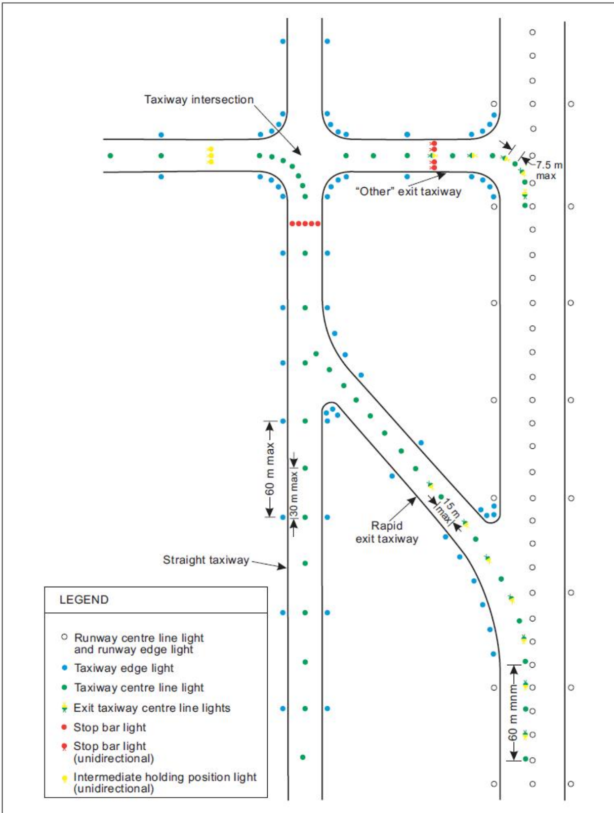
Figure M-11. Taxiway lighting
