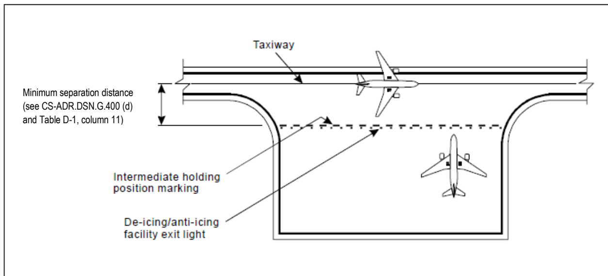
Figure M-12. Example of remote de-icing/anti-icing facility
