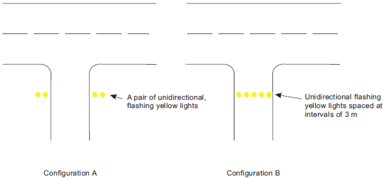
Figure M-13. Runway guard lights
