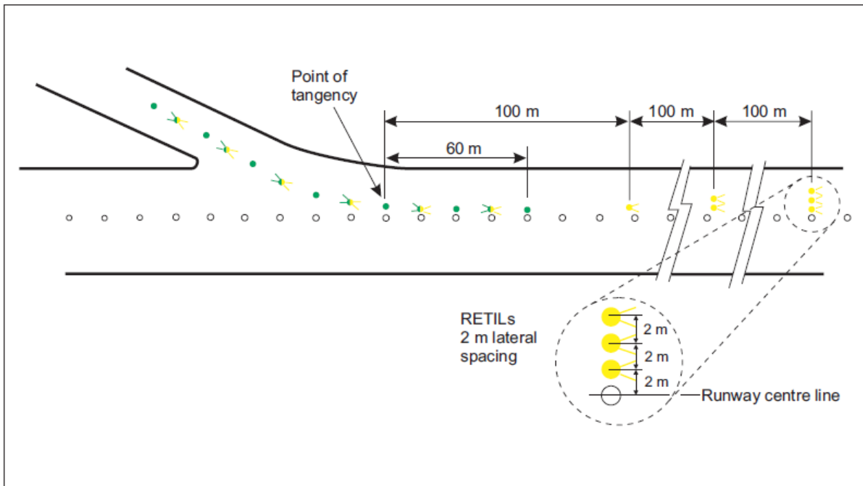
Figure M-9. Rapid exit taxiway indicator lights (RETILs)
