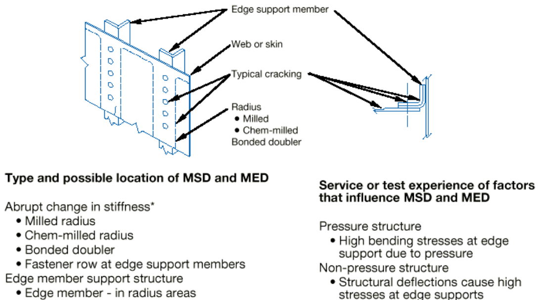
Figure A2-9 Abrupt Changes in Web or Skin Thickness — Pressurised or Unpressurised Structure (MSD/MED)
