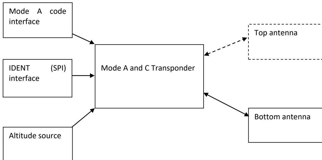
Figure 2: Mode A/C transponder interfaces
