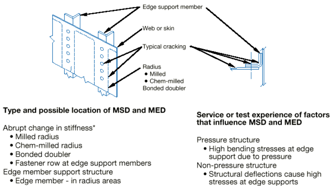
Figure A2-9 Abrupt Changes in Web or Skin Thickness — Pressurised or Unpressurised Structure (MSD/MED)
