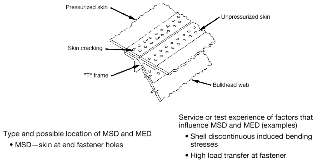
Figure A2-8 Skin Splice at Aft Pressure Bulkhead (MSD)
