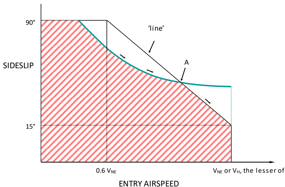
Figure 1 — YAW/FORWARD SPEED DIAGRAM
