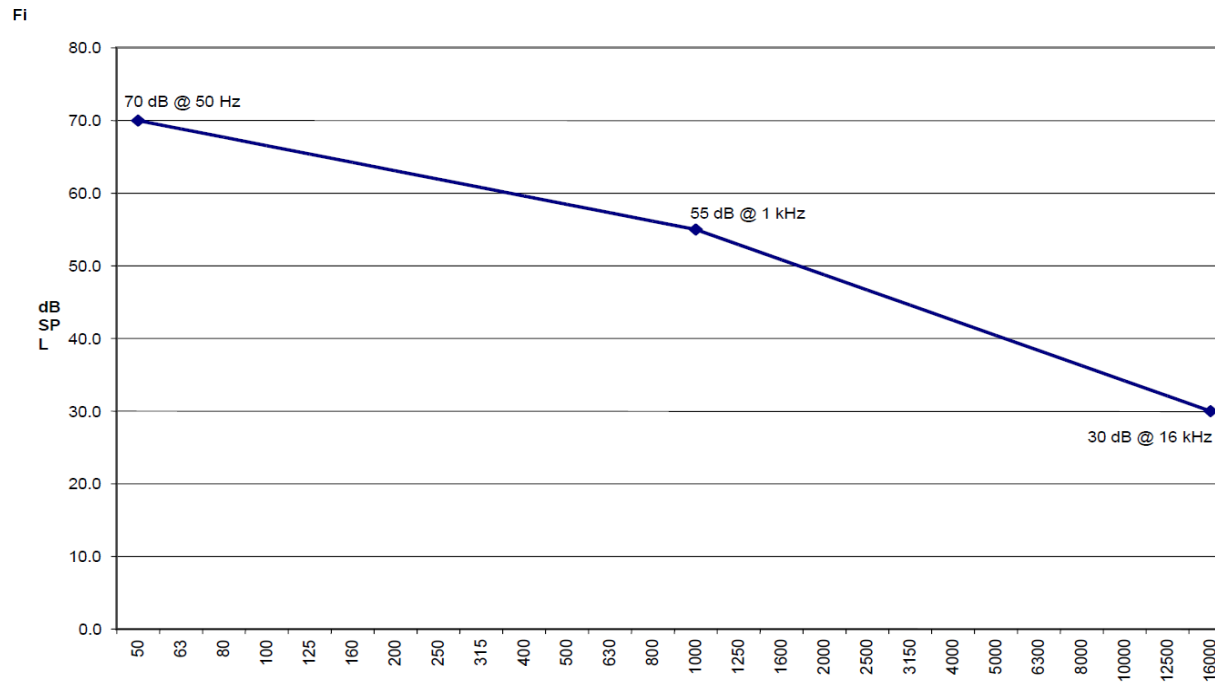
Figure 3: 1/3 octave band frequency (Hz)
