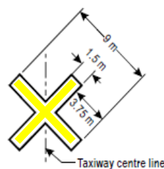
Illustration b) Closed taxiway marking
