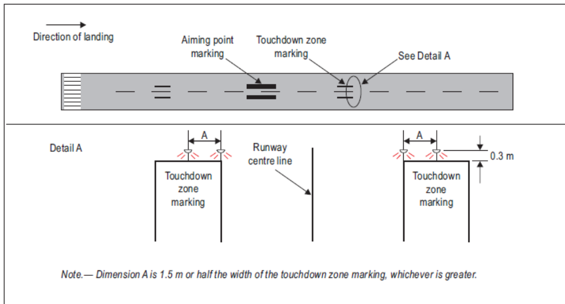
Figure M-8(C). Simple touchdown zone lighting
