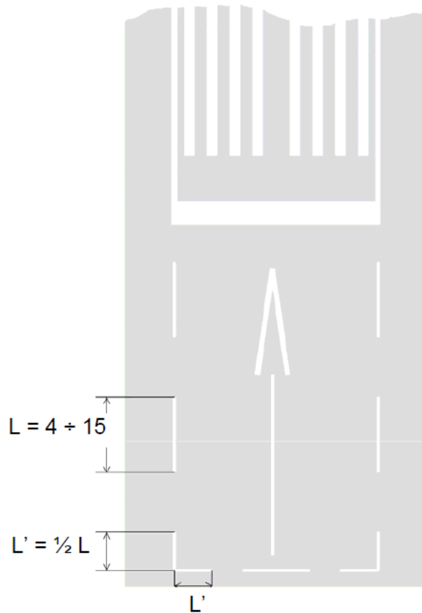
Figure GM-L-1. Dashed runway side stripe marking
