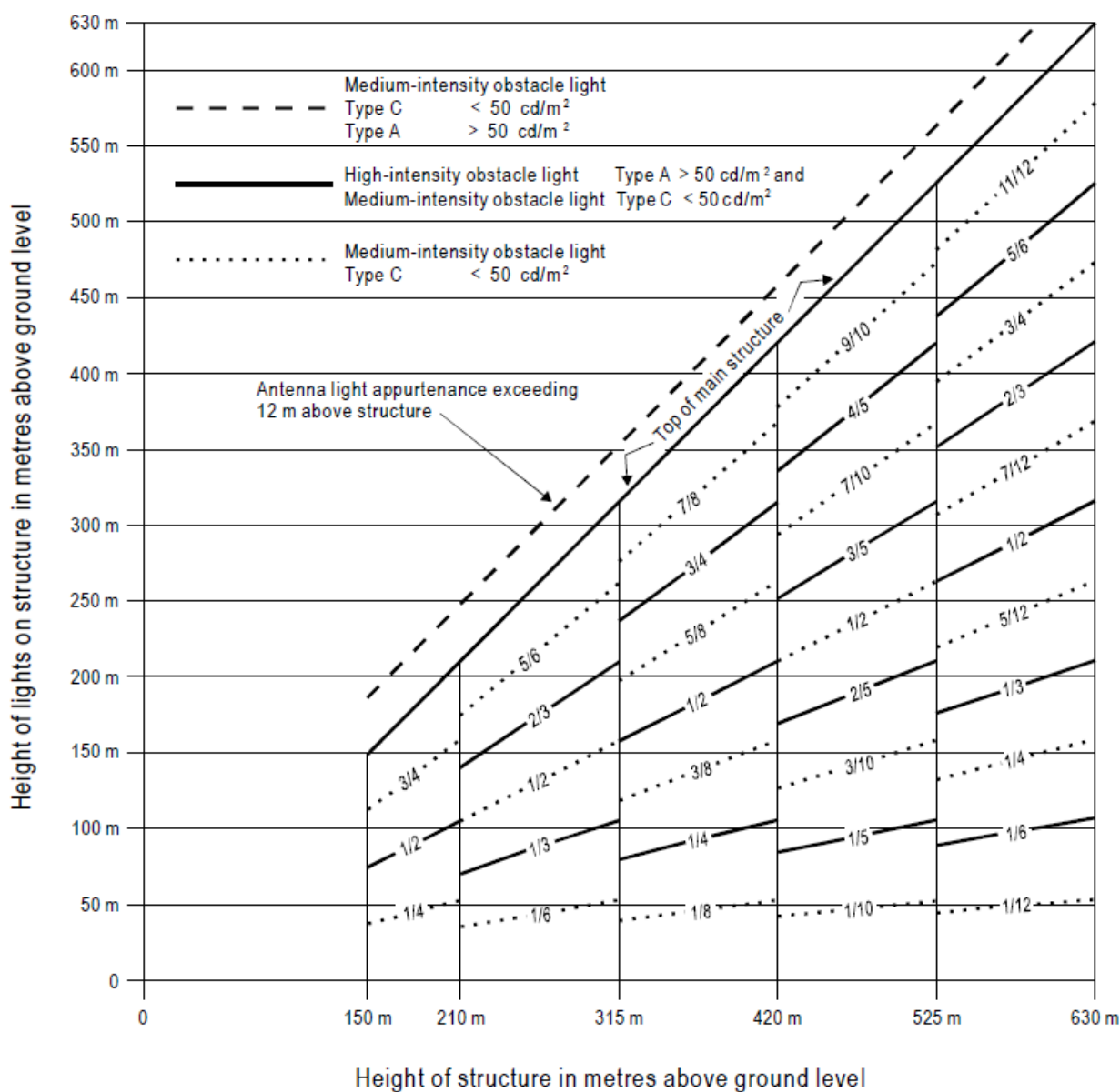
Figure GM-Q-8. High-/medium-intensity dual obstacle lighting system, Type A/Type C
