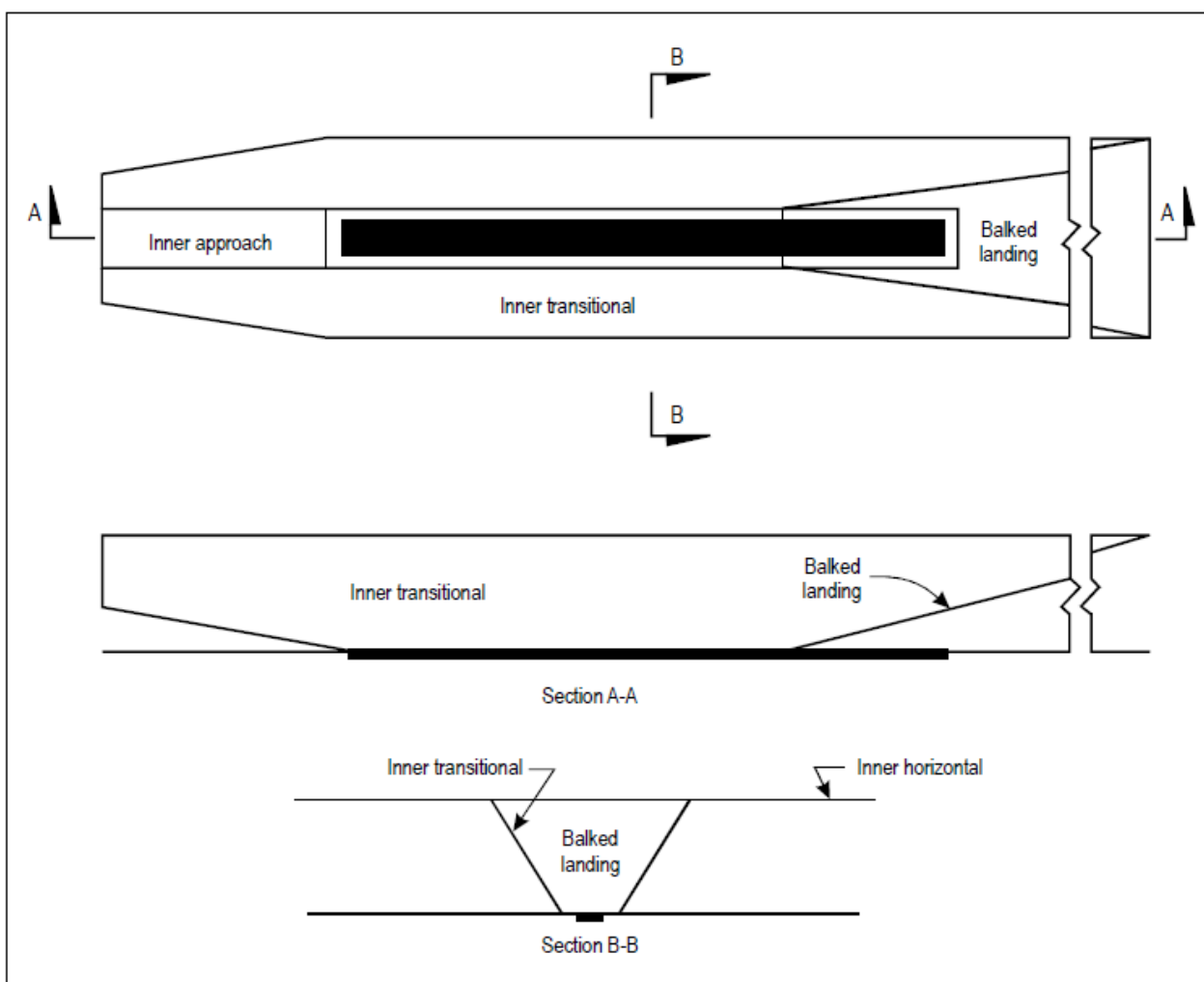
Figure H-3. Inner approach, inner transitional, and bailed landing obstacle limitation surfaces
