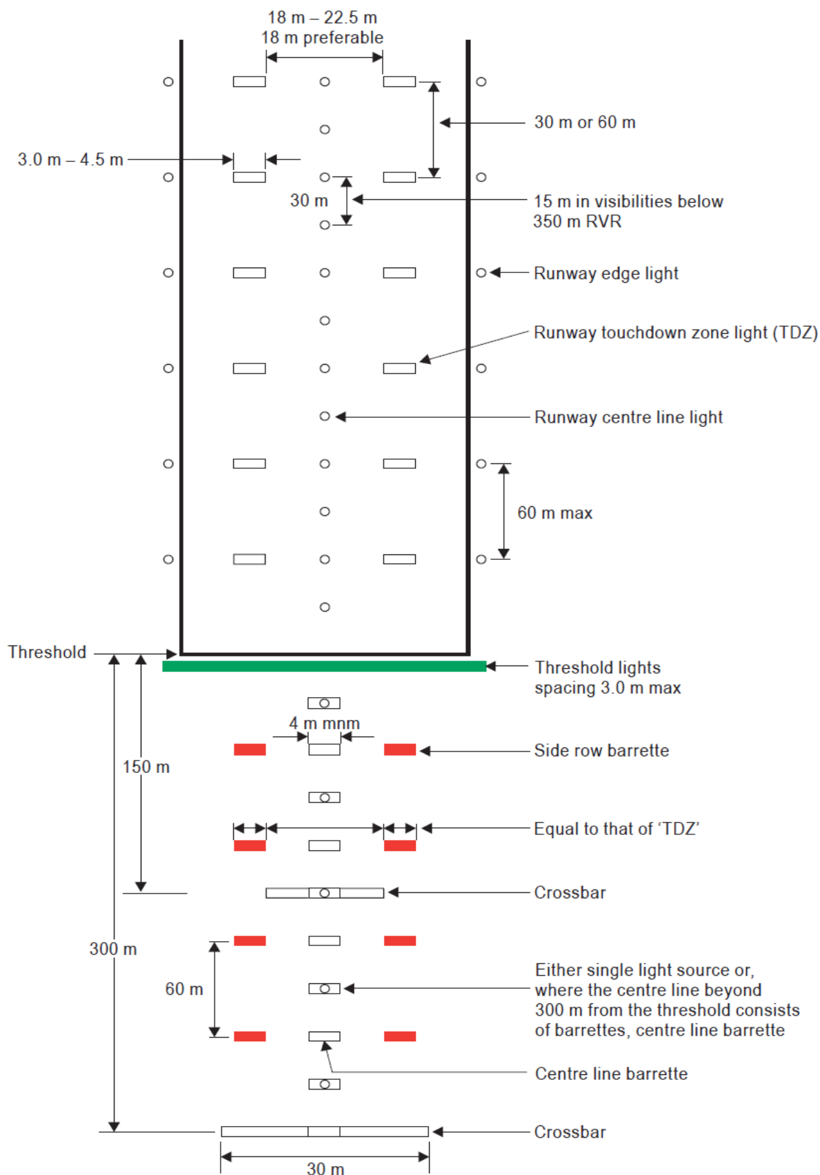
Figure M-3B. Inner 300m approach and runway lighting for precision approach runways, Categories II and III where the serviceability levels of the lights specified as maintenance objectives in CS ADR-DSN.S.895 can be demonstrated
