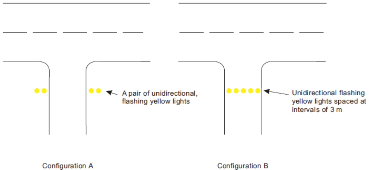
Figure M-12. Runway guard lights
