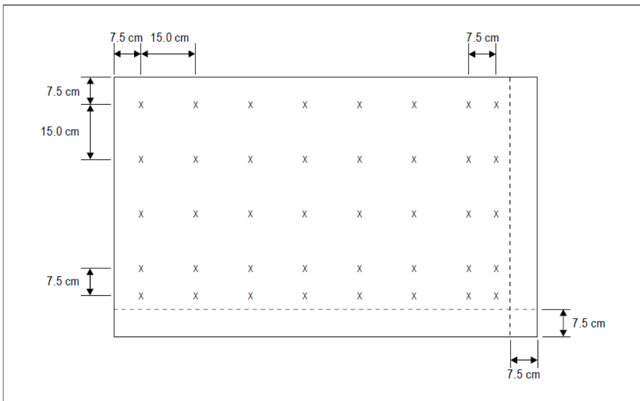
Figure N-1. Grid points for calculating average luminance of a sign
