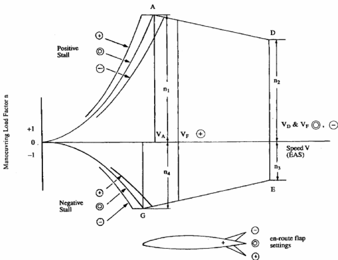
FIGURE 1 MANOEUVRING ENVELOPE
