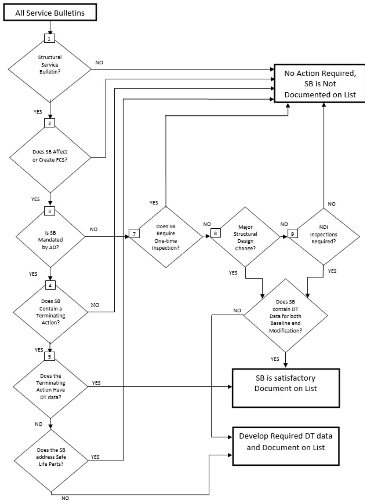
Figure A3(4)-1. Service Bulletin (SB) Flow Chart
