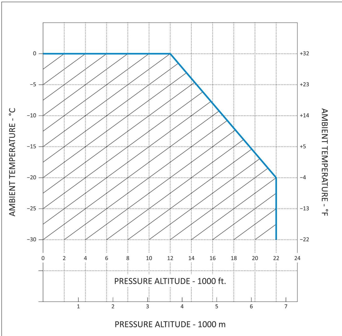
FIGURE 2 CONTINUOUS MAXIMUM (STRATIFORM CLOUDS) ATMOSPHERIC ICING CONDITIONS AMBIENT TEMPERATURE VS PRESSURE ALTITUDE
