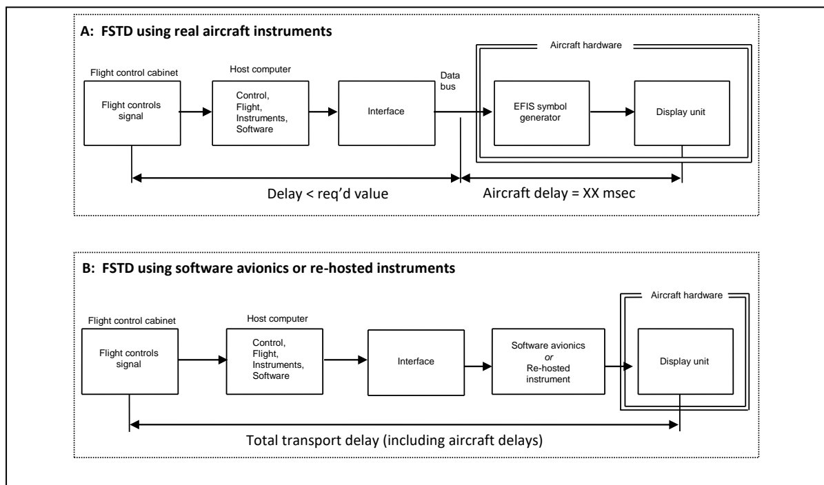
Figure 4A and 4B: Transport delay for simulation of aircraft using real or re-hosted instrument drivers
