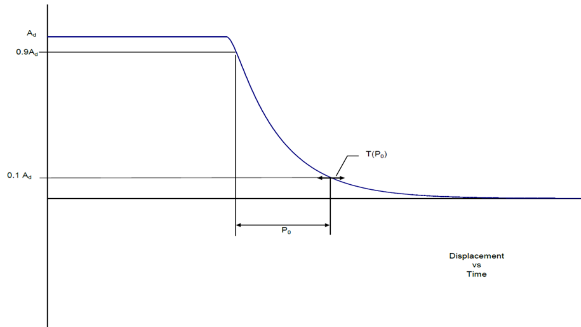
Figure 2: Critically damped step response
