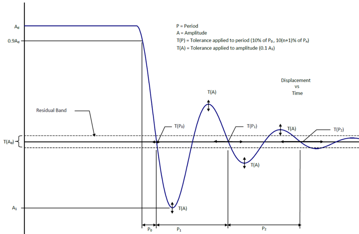
Figure 1: Underdamped step response
