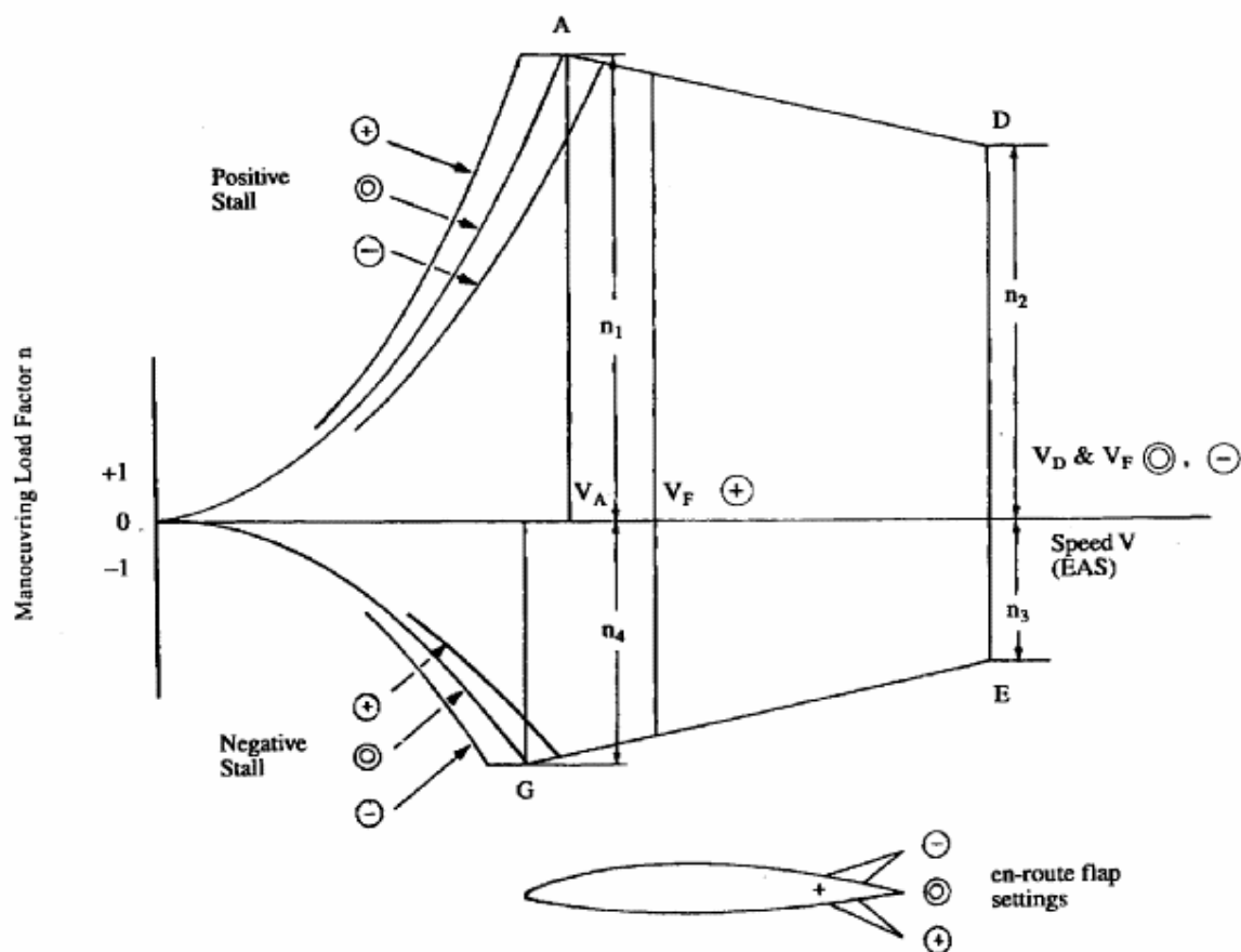
FIGURE 1 MANOEUVRING ENVELOPE
